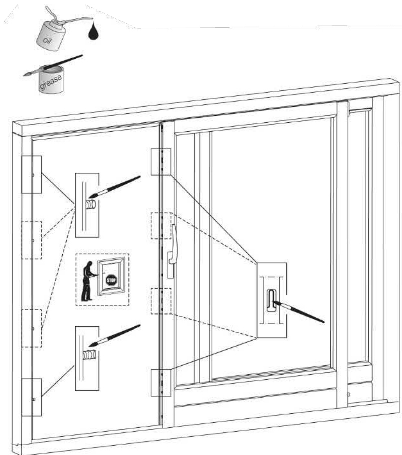
Abb.67: Wartung Hebeschiebetüren Fig.67: Maintenance lifting sliding systems
